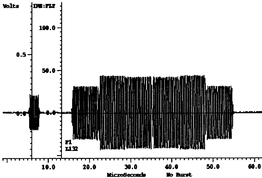
Figure 58. 100/75% Color Bars NTSC (Chrominance Only)
