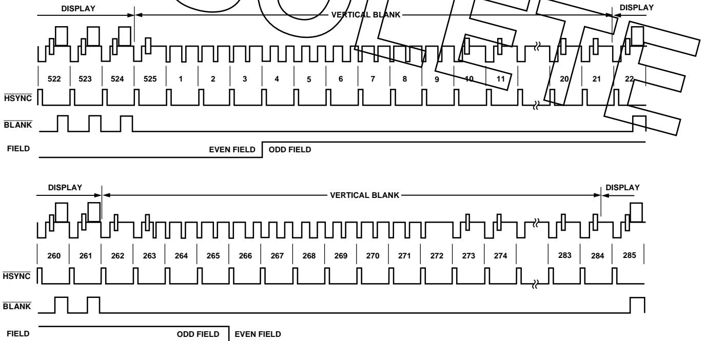
Figure 24. Timing Mode 3 (NTSC)
