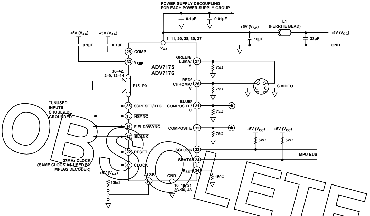
Figure 41. Recommended Analog Circuit Layout
